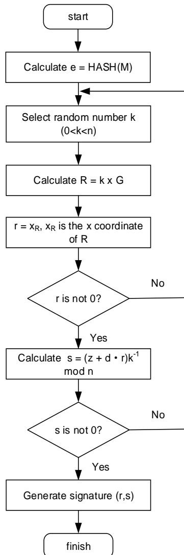
Figure 11-3. Flow chart of ECDSA sign
