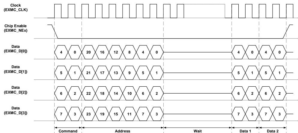
Figure 30-26. QPI-PSRAM access
