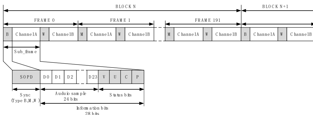
Figure 26-15 SPDIF data formate
