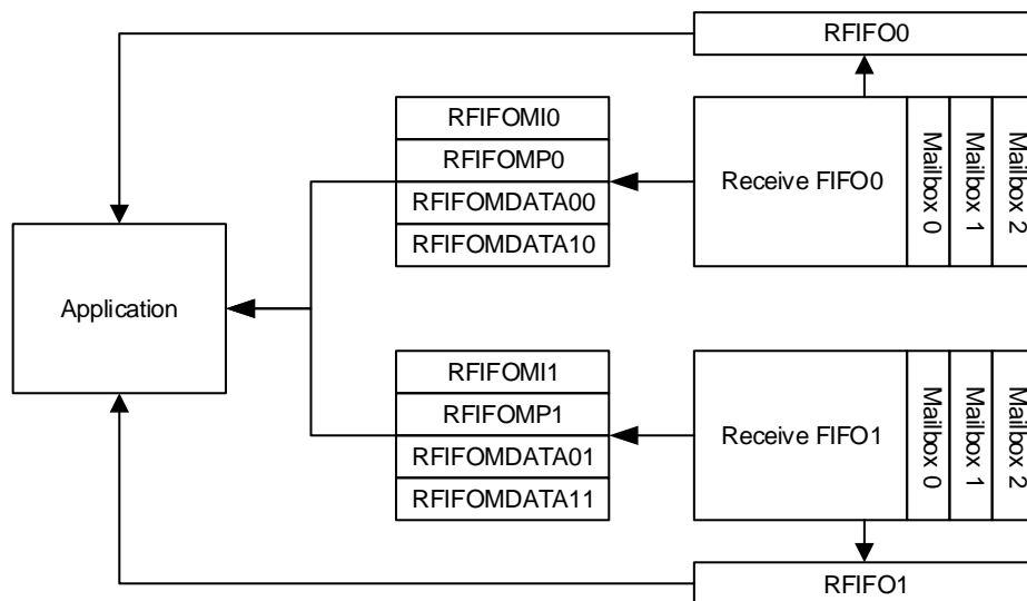
Figure 31-4. Reception register
