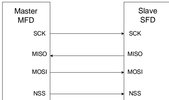
Figure 25-5. A typical simplex connection (Master: Receive, Slave: Transmit)
