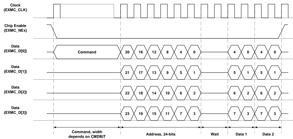
Figure 30-25. SQPI-PSRAM access
