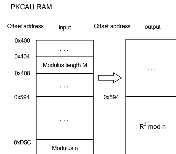
Figure 11-12. Montgomery parameter calculation
