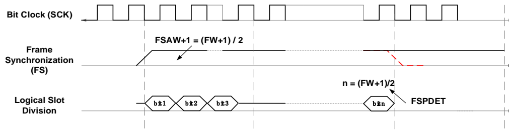
Figure 26-19 Frame synchronization postponed detection
