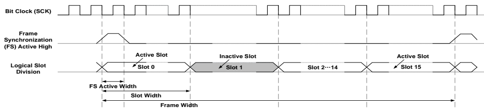
Figure 26-6 Slot activation
