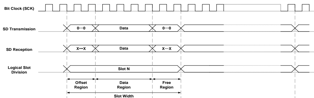
Figure 26-12 Data configuration
