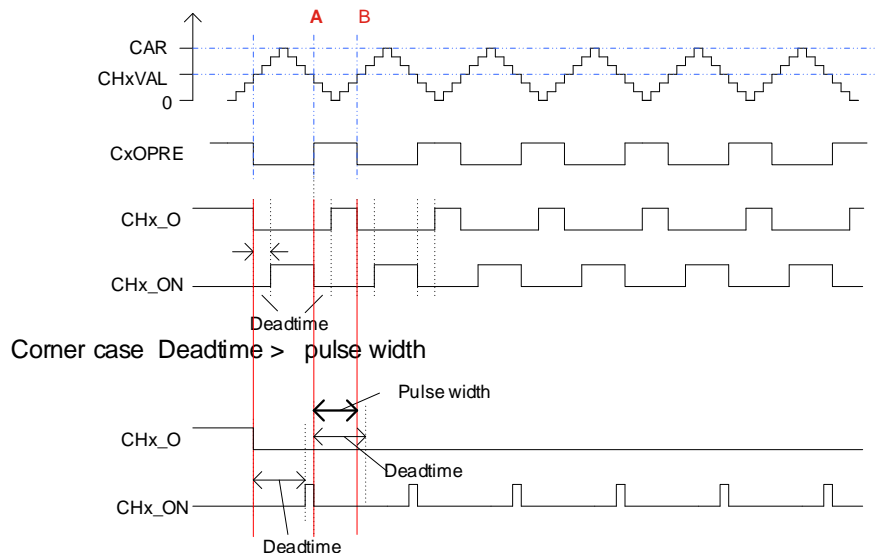
Figure 22-22. Complementary output with dead-time insertion.
