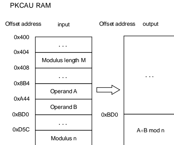
Figure 11-10. Modular addition
