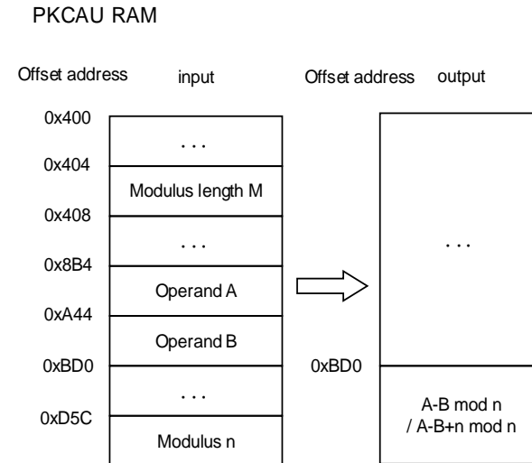
Figure 11-11. Modular subtraction
