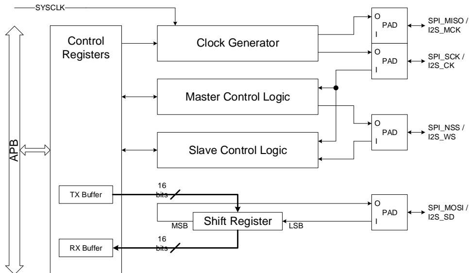
Figure 25-13. Block diagram of I2S
