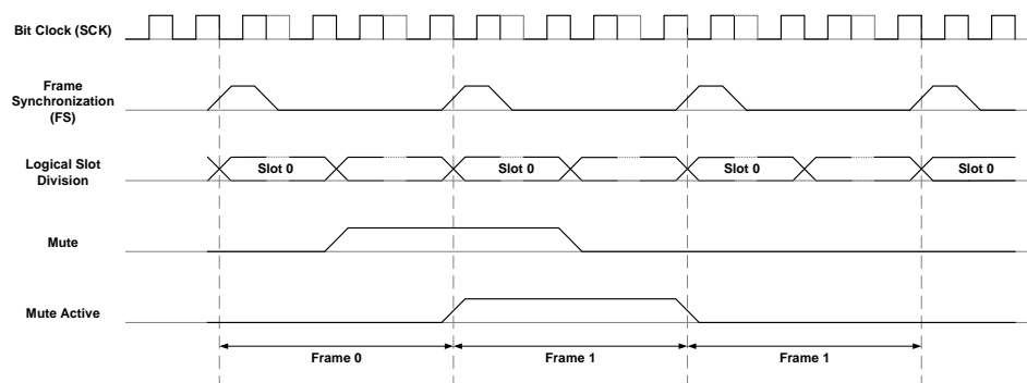
Figure 26-16 Mute frame activation
