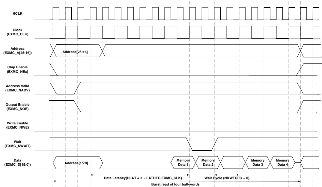
Figure 30-22. Read timing of synchronous multiplexed burst mode
