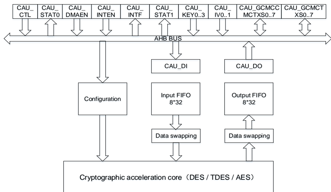
Figure 13-3. CAU diagram
