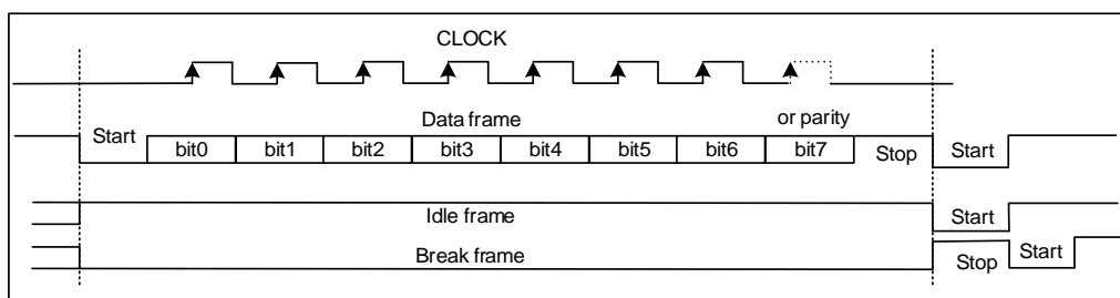
Figure 23-2. USART character frame (8 bits data and 1 stop bit)
