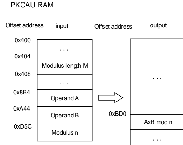
Figure 11-14. Montgomery multiplication
