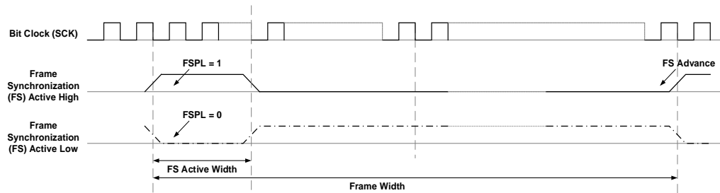
Figure 26-4 FS polarity
