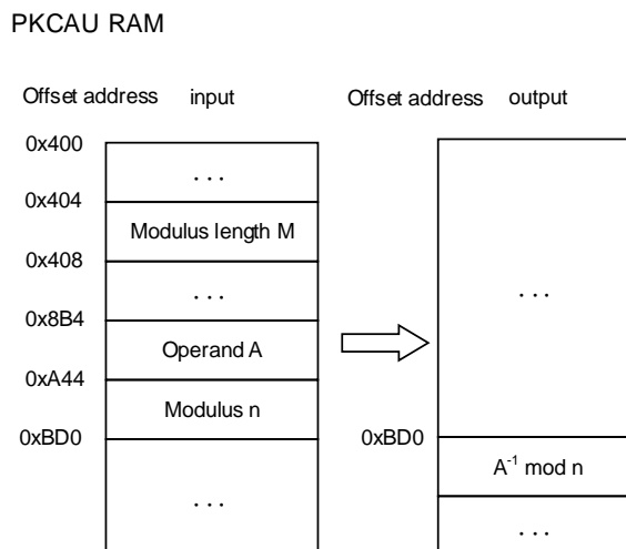
Figure 11-17. Modular inversion
