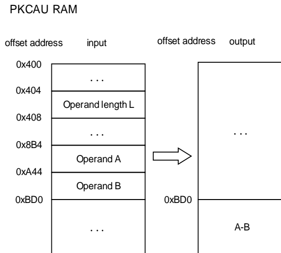
Figure 11-6. Arithmetic subtraction
