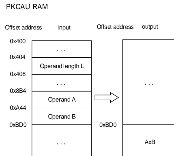
Figure 11-7. Arithmetic multiplication
