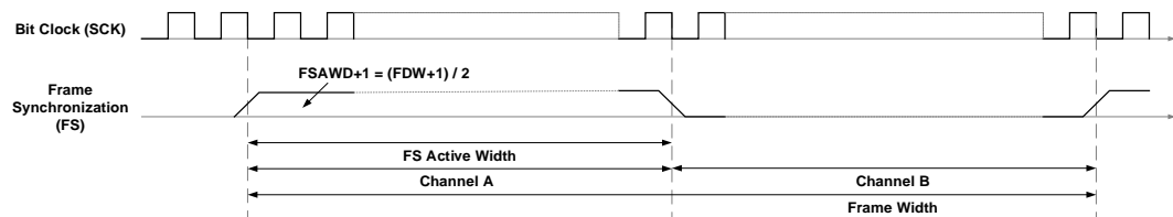
Figure 26-5 FS function
