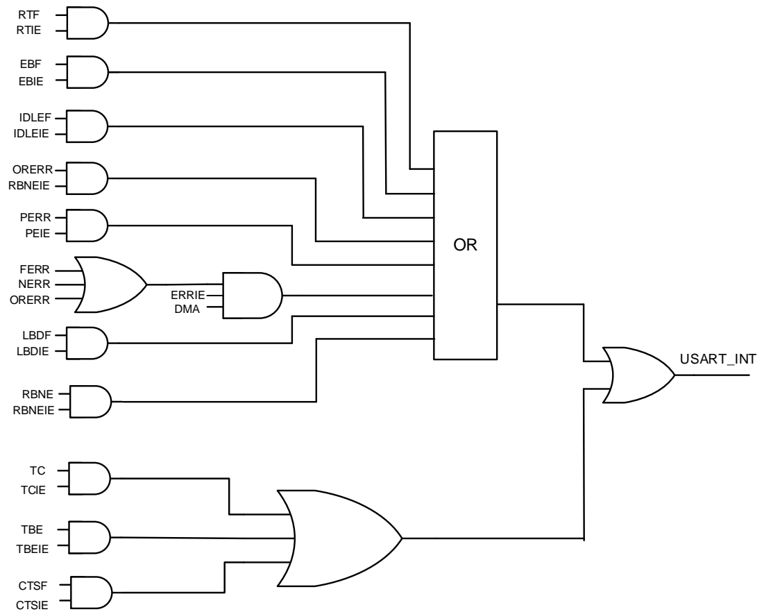
Figure 23-16. USART interrupt mapping diagram
