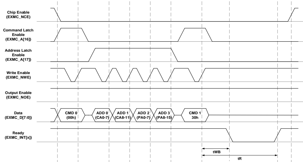
Figure 30-28. Access to none "NCE don't care" NAND Flash
