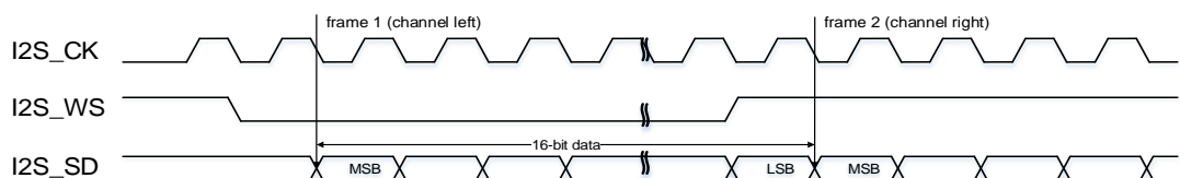
Figure 25-14. I2S Philips standard timing diagram (DTLEN=00, CHLEN=0, CKPL=0)
