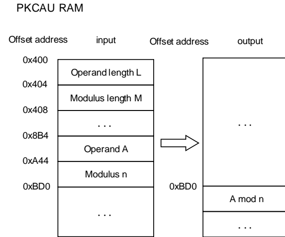
Figure 11-9. Modular reduction
