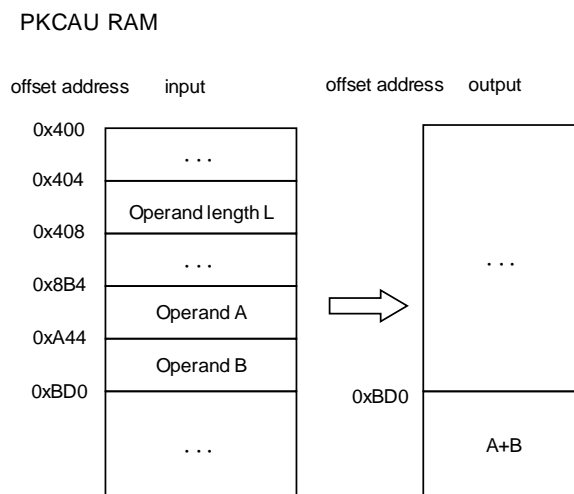
Figure 11-5. Arithmetic addition
