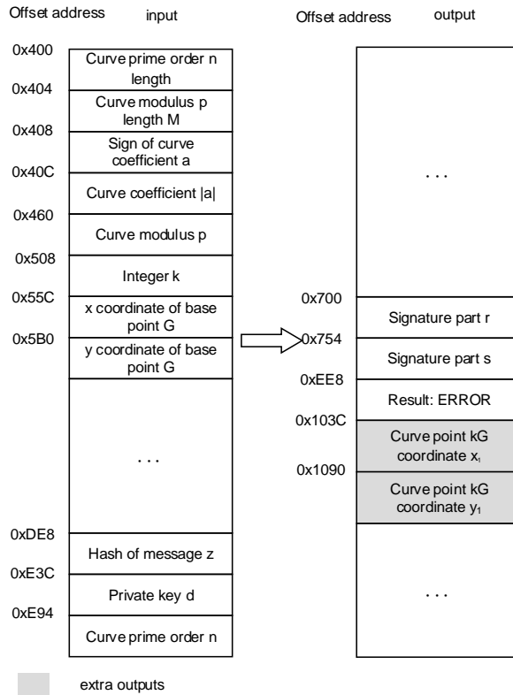
Figure 11-22. ECDSA sign
