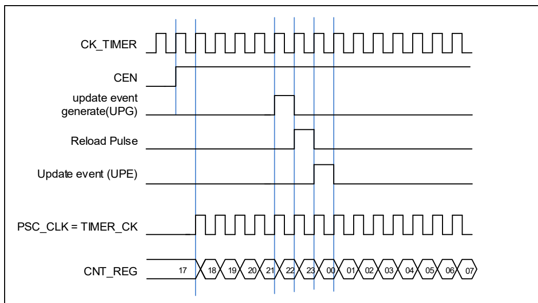
Figure 16-66. Timing chart of internal clock divided by 1
