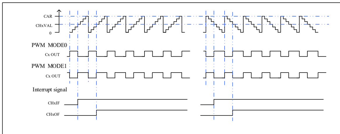
Figure 16-52. EAPWM timechart
