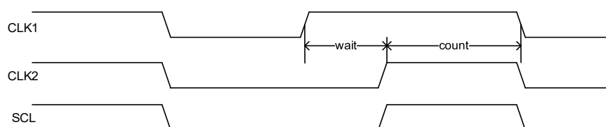
Figure 18-4. Clock synchronization
