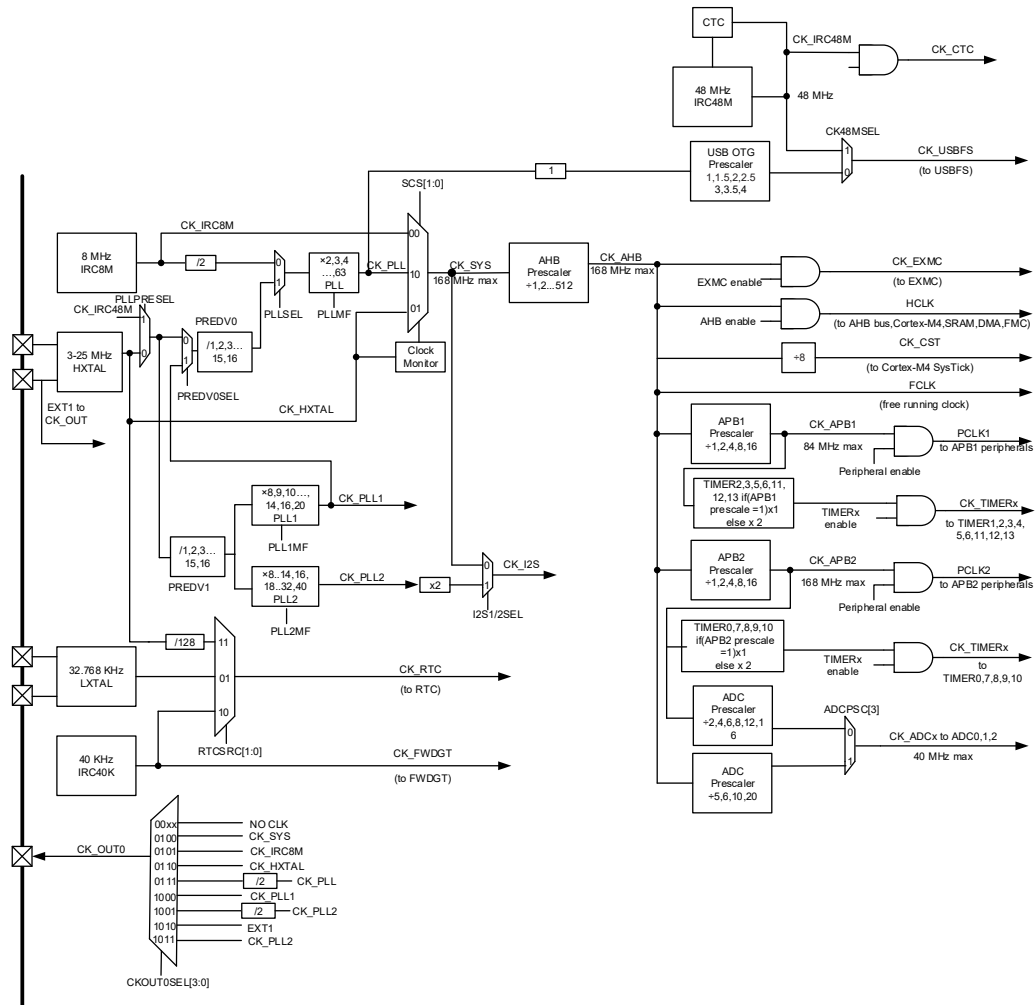
Figure 5-2. Clock tree
