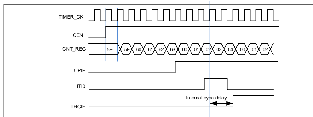
Figure 16-22. Restart mode
