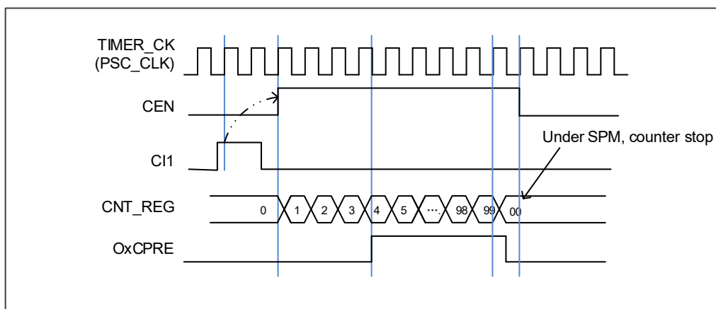
Figure 16-57. Single pulse mode TIMERx\_CHxCV = 4 TIMERx\_CAR=99
