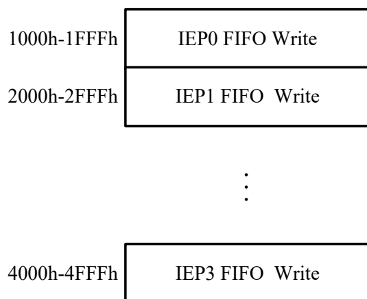
Figure 23-8. Device mode FIFO access register map
