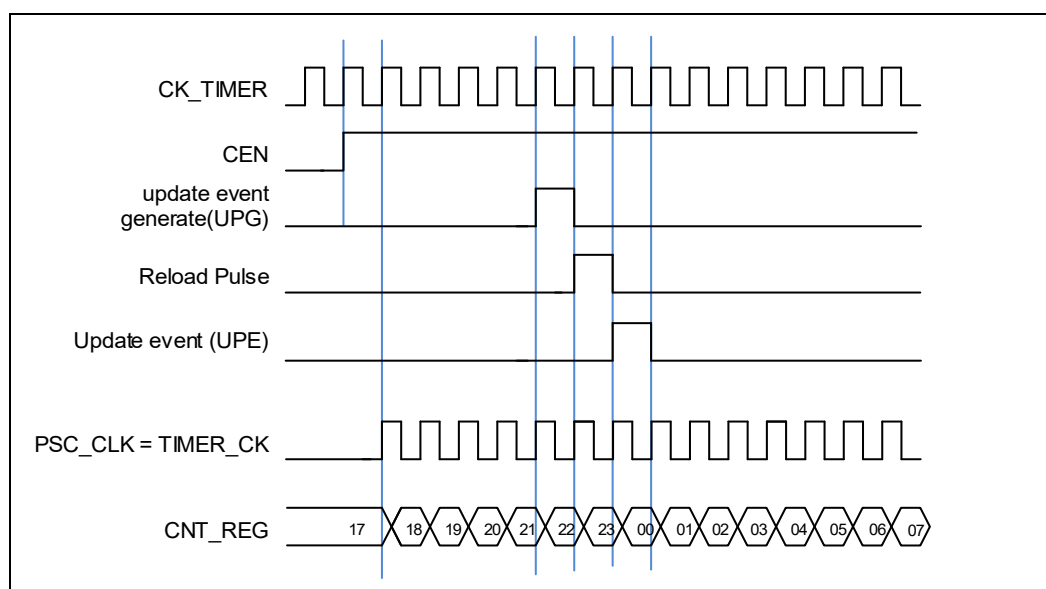
Figure 16-59. Timing chart of internal clock divided by 1
