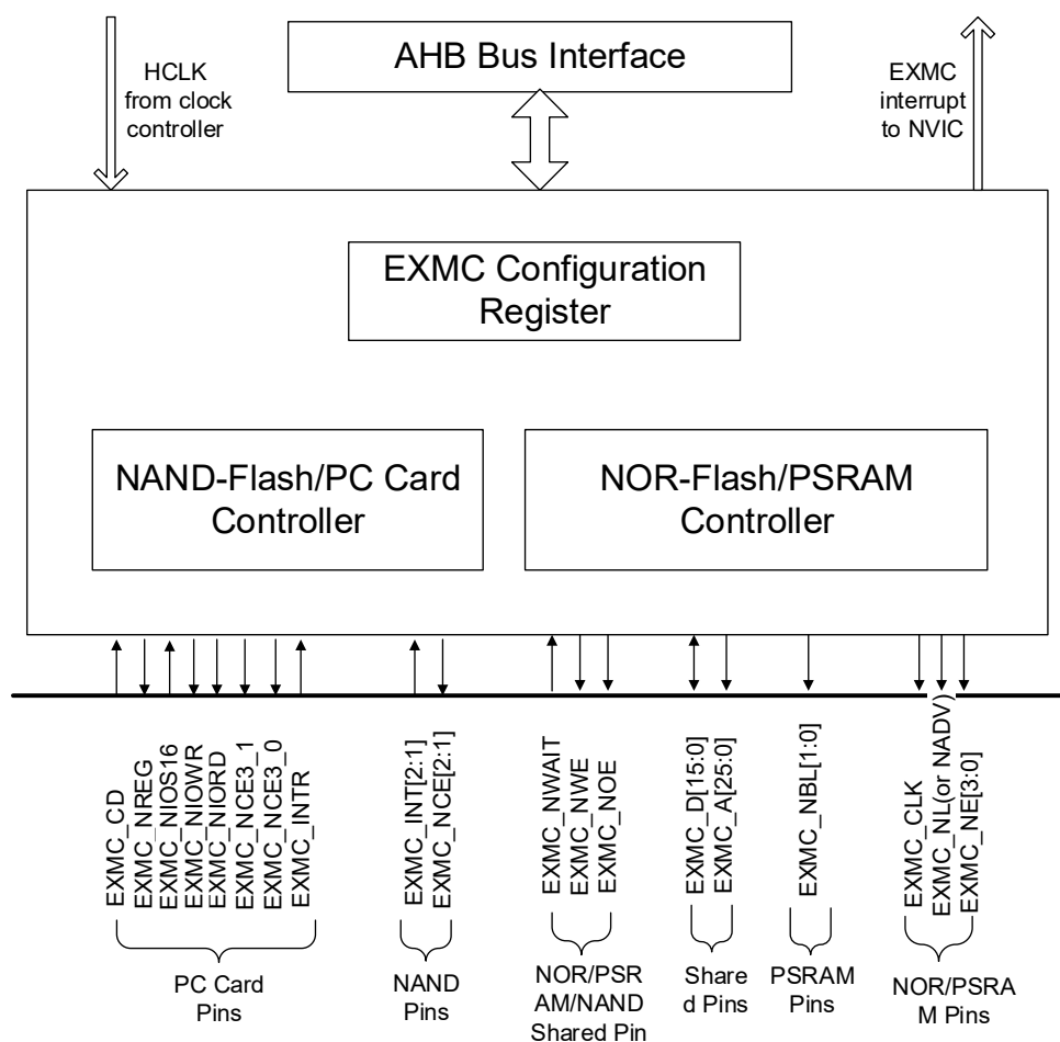
Figure 21-1. The EXMC block diagram
