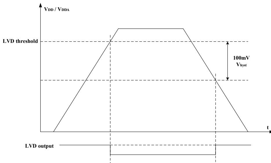
Figure 3-3. Waveform of the LVD threshold
