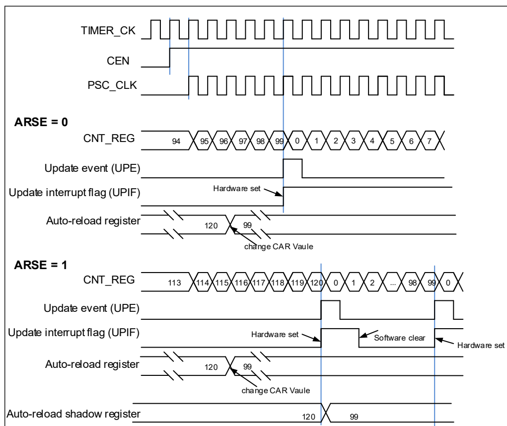
Figure 16-62. Timing chart of up counting mode, change TIMERx_CAR on the go
