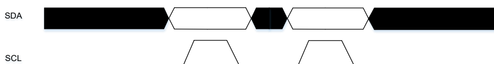
Figure 18-2. Data validation
