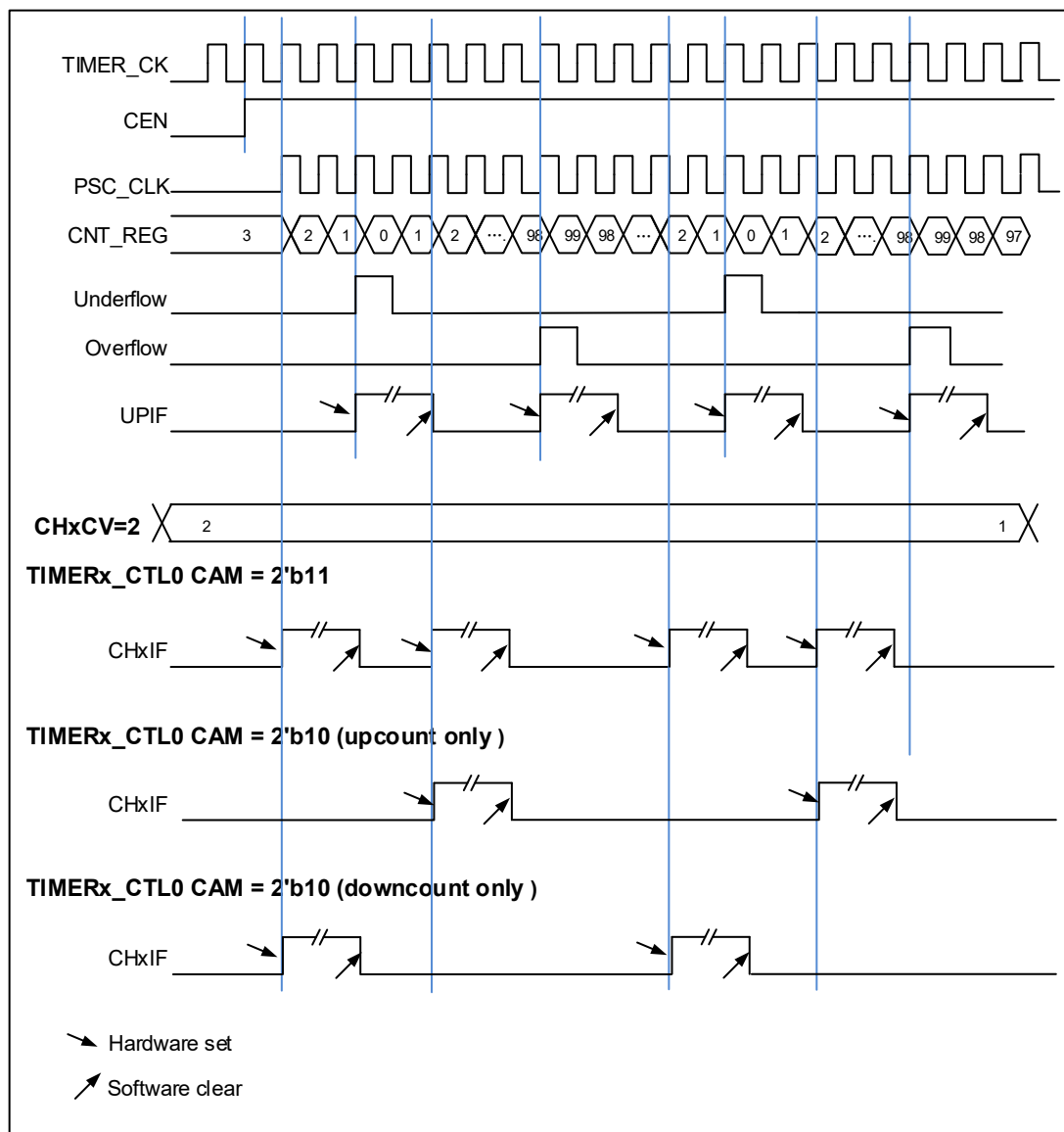
Figure 16-8. Timing chart of center-aligned counting
