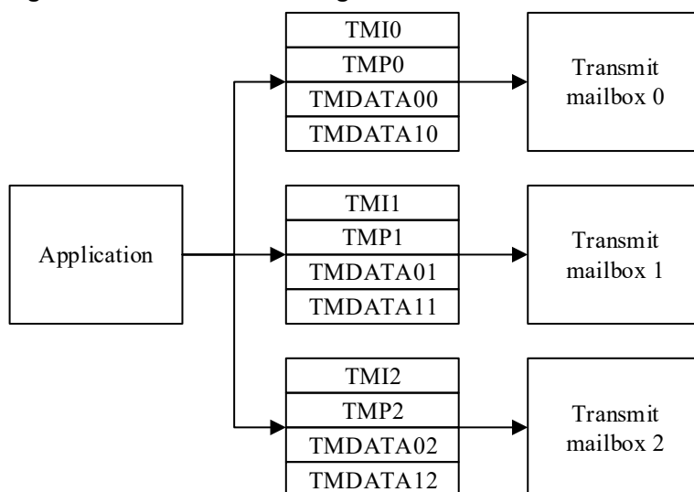
Figure 22-2. Transmission register
