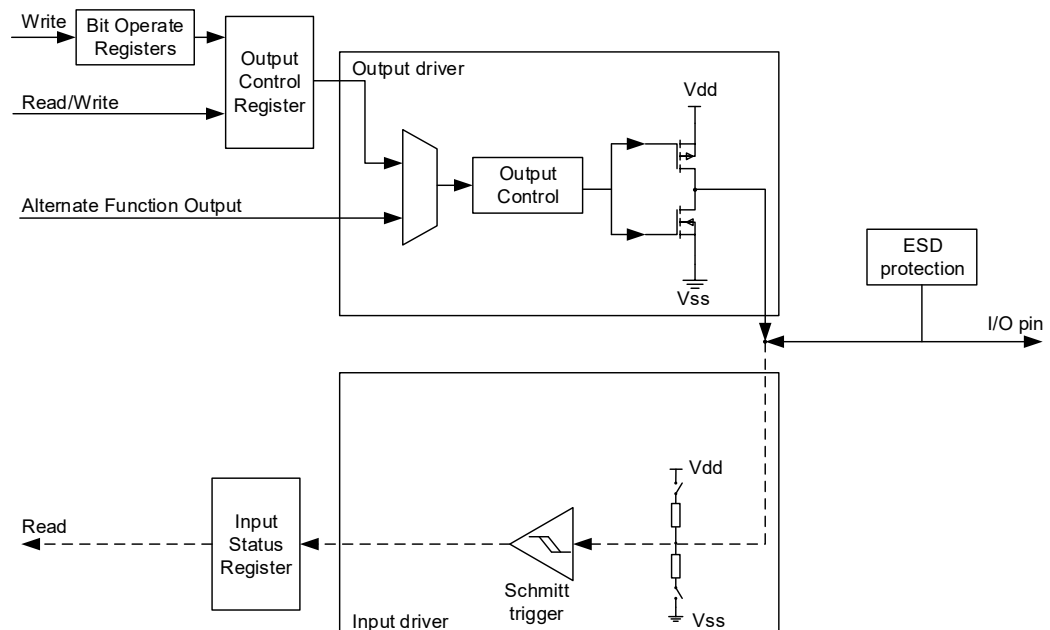
Figure 8-3. Output configuration
