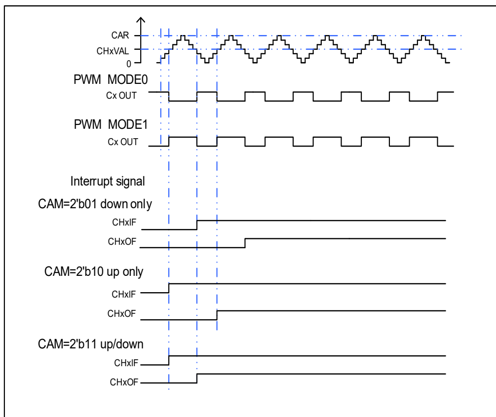
Figure 16-53. CAPWM timechart
