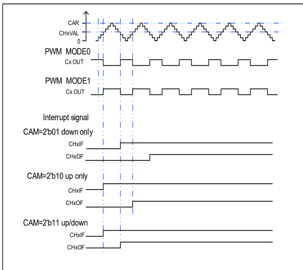
Figure 16-15. CAPWM timechart
