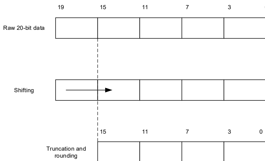
Figure 12-9. 20-bit to 16-bit result truncation
