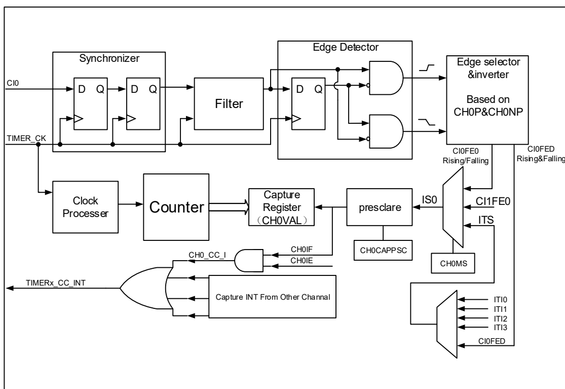
Figure 16-50. Channels input capture principle
