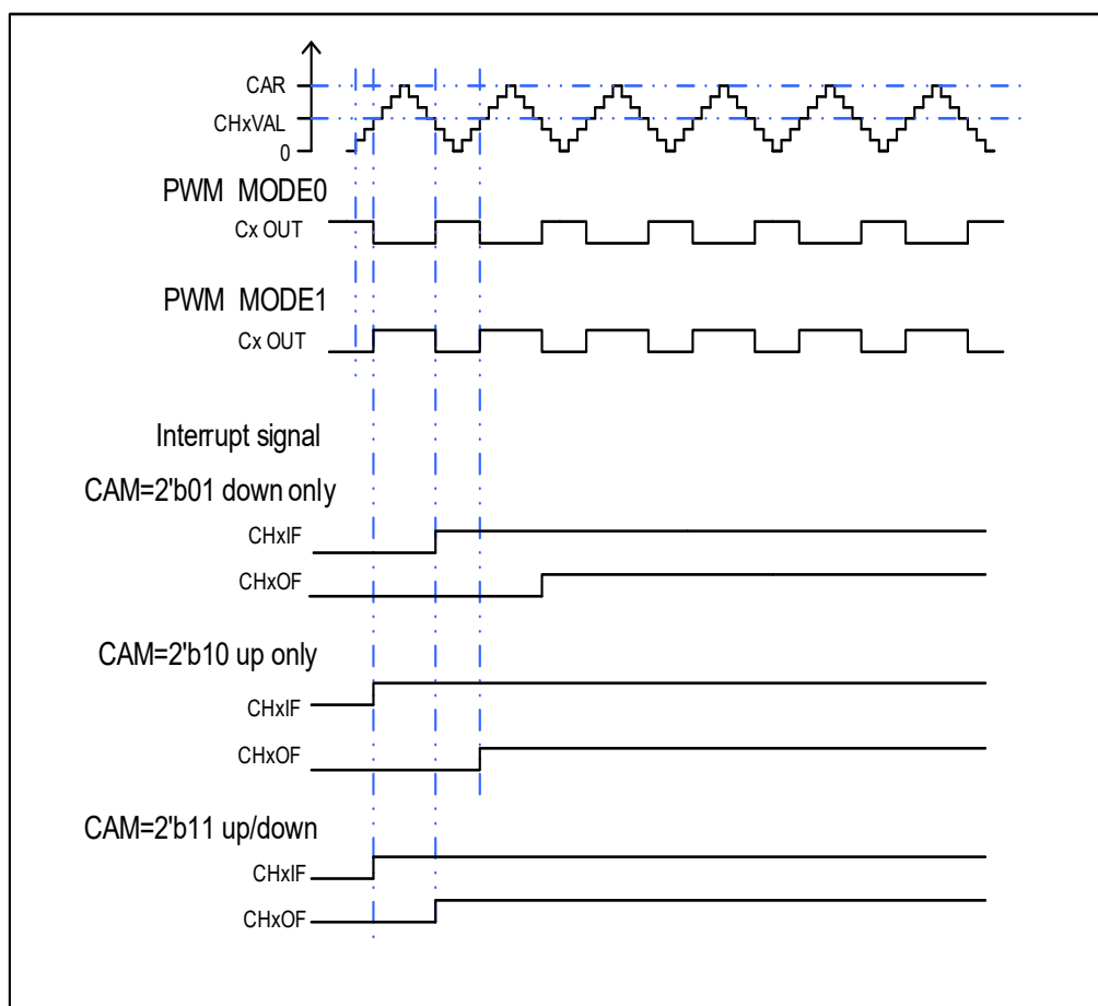
Figure 16-15. CAPWM timechart
