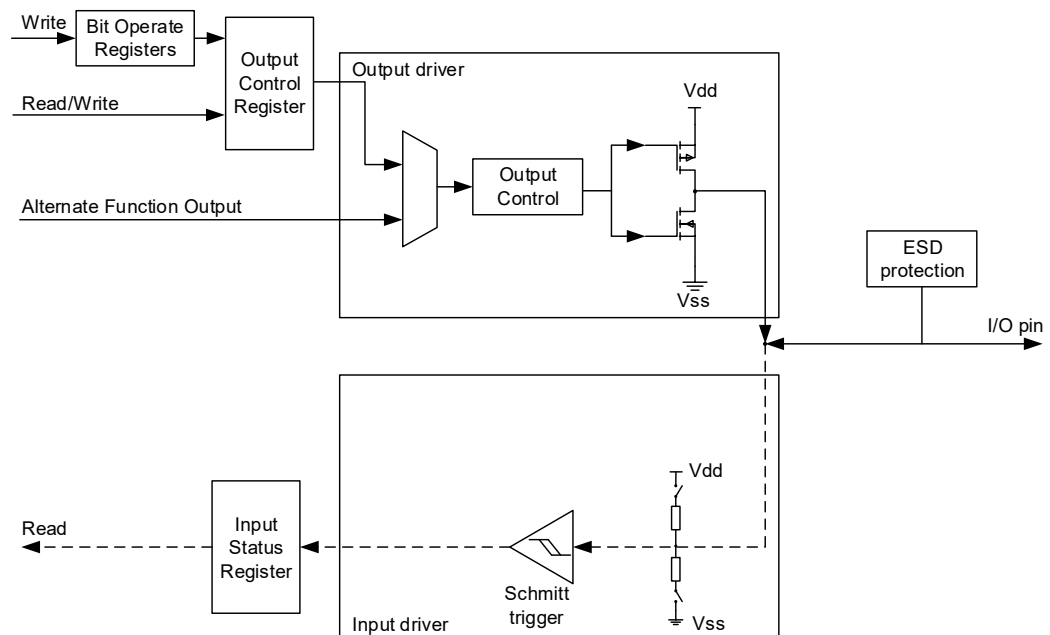
Figure 8-3. Output configuration
