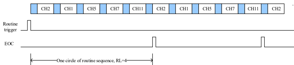
Figure 12-5. Scan operation mode, continuous enable
