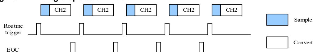
Figure 12-2. Single operation mode
