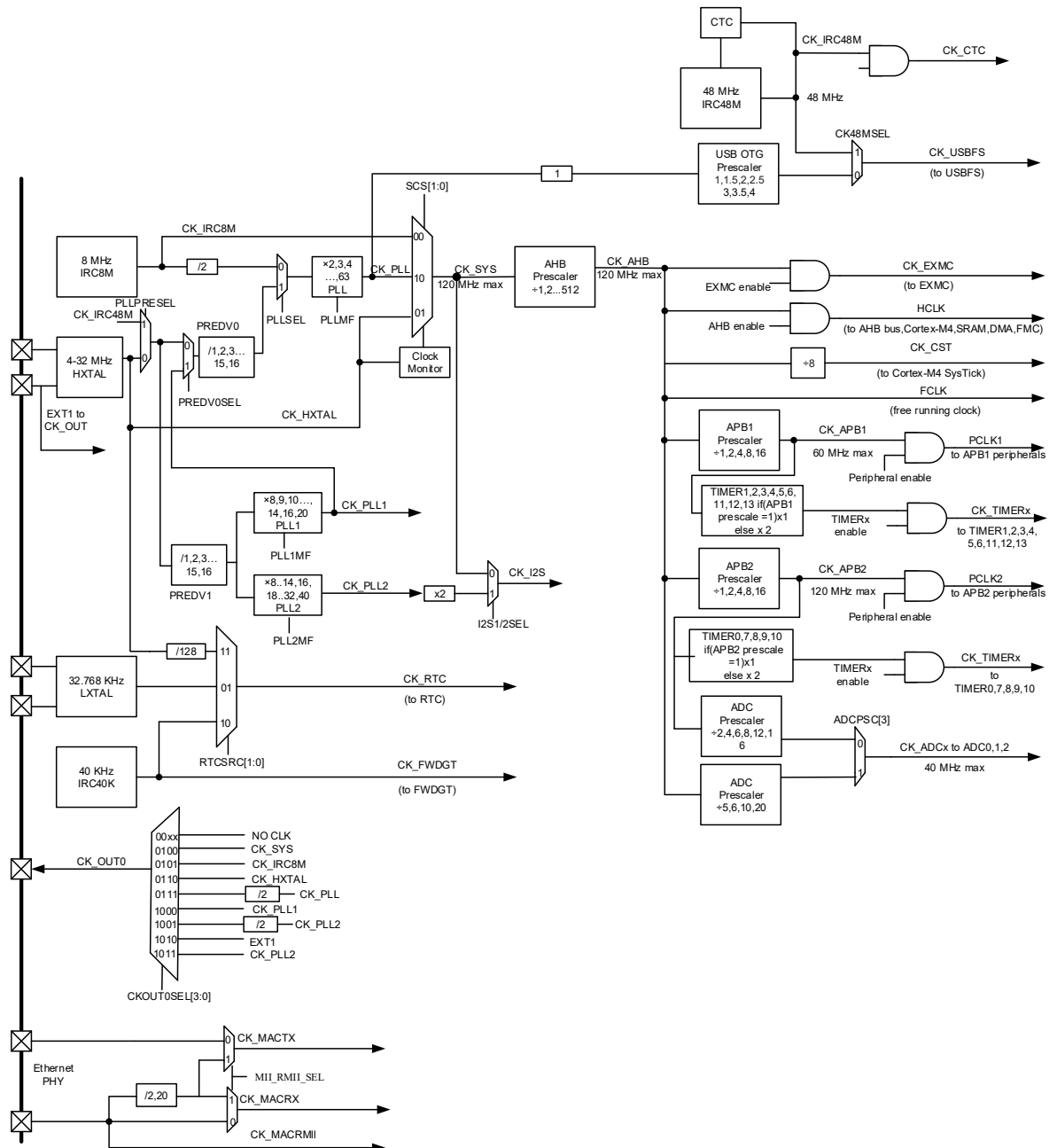
Figure 5-6. Clock tree
