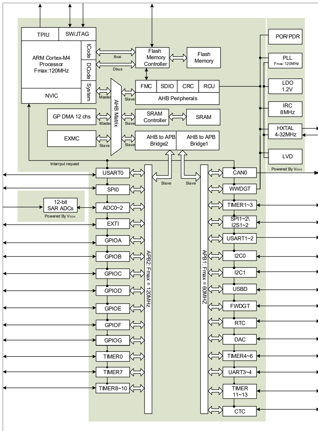
Figure 1-2. GD32F303 series system architecture
