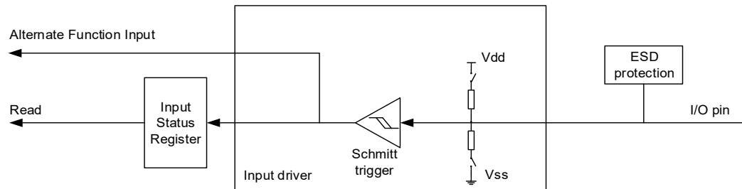
Figure 8-2. Input configuration
