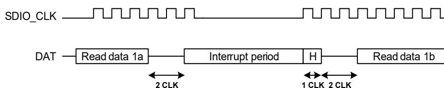
Figure 20-12. Read wait control by stopping SDIO_CLK
