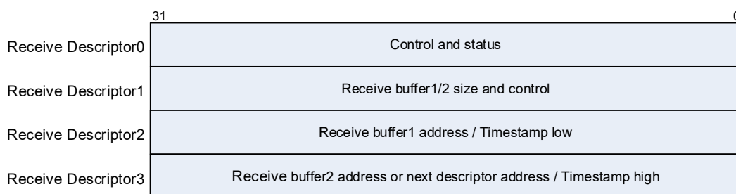
Figure 23-9. Receive descriptor in normal mode
