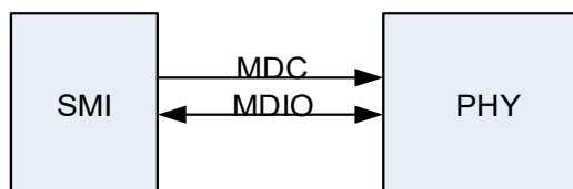
Figure 23-3. Station management interface signals
