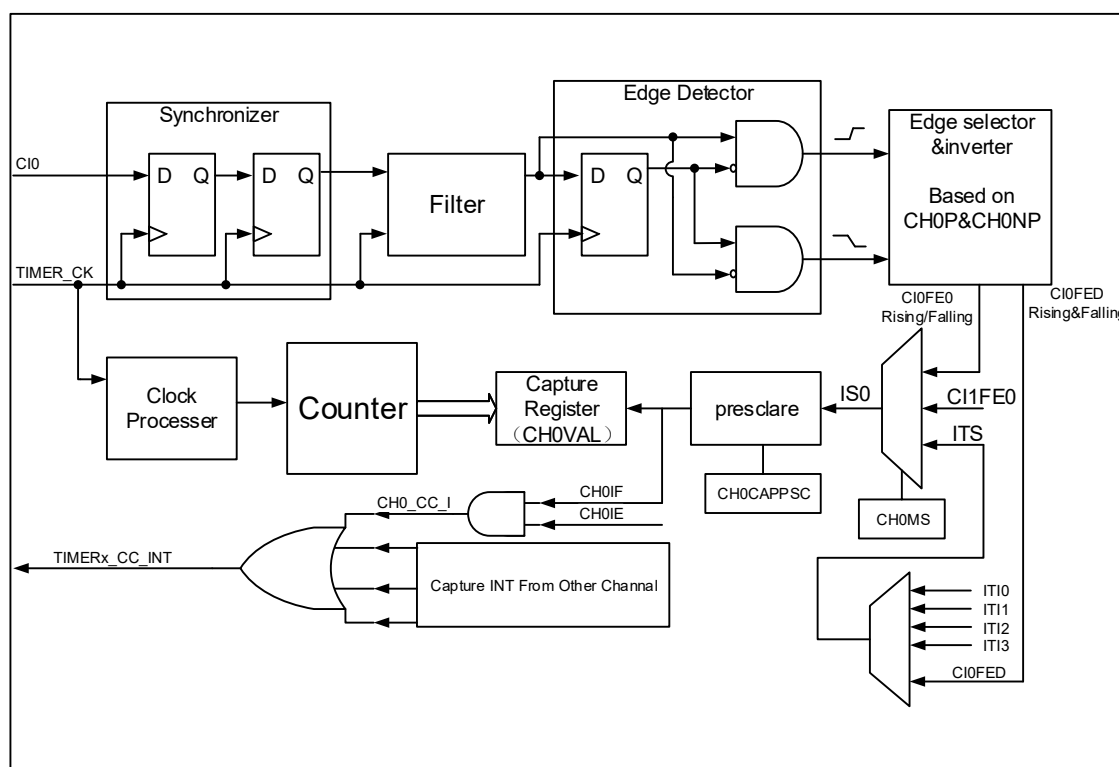
Figure 16-62. Channel input capture principle
